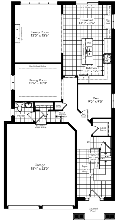
Ground Floor Elevation A
