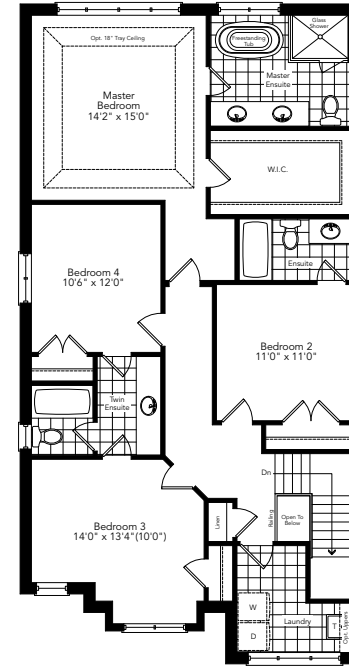
Second Floor Optional 3 Bath Plan Elevation A
