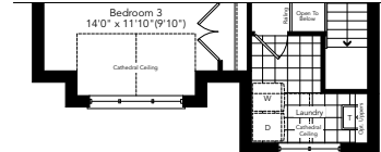
Second Floor Optional 3 Bath Plan Elevation A
