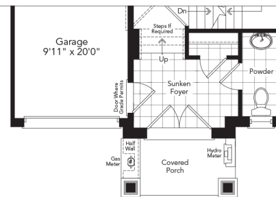
Partial Ground & Optional Ground Floor Elevation B
