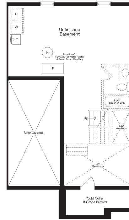
Basement For Optional Ground Floor Elevation A
