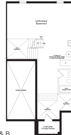
Basement Elevation A & B
