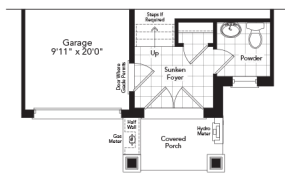
Partial Ground Floor Elevation B
