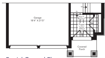
Partial Ground Floor Elevation C
