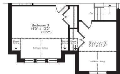
Partial Second Floor Elevation B
