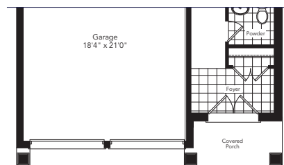
Partial Ground Floor Elevation B
