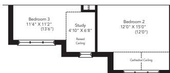
Partial Second Floor Elevation C
