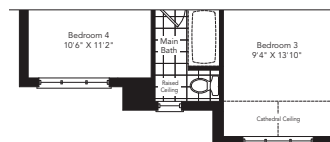
Partial Second Floor Optional 4 Bedroom Plan Elevation C
