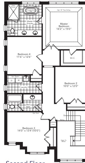
Second Floor Elevation A
