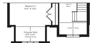
Partial Second Floor Elevation C
