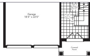
Partial Ground Floor Elevation C
