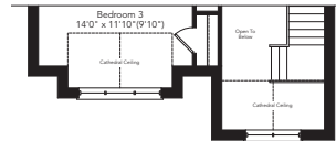
Partial Second Floor Elevation C
