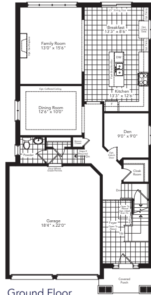
Ground Floor Elevation A
