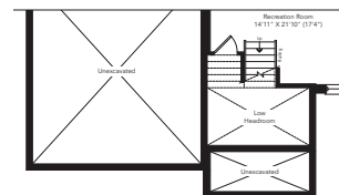
Partial Basement Elevation C
