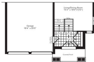
Partial Ground Floor Elevation B
