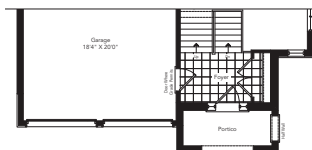
Partial Ground Floor & Partial Optional Ground Floor Elevation C
