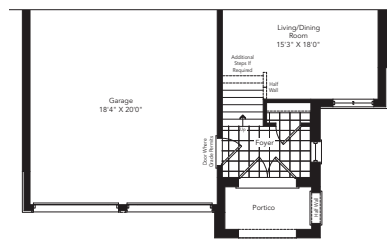
Partial Ground Floor & Partial Optional 3 Bedroom Plan Elevation C
