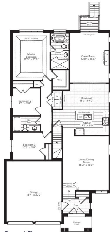
Ground Floor Optional 3 Bedroom Plan Elevation A
