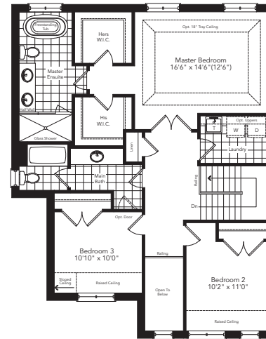
Second Floor Elevation A
