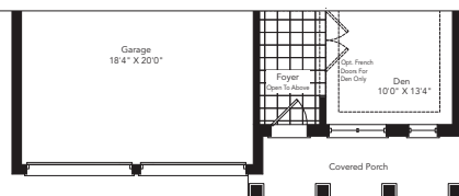
Partial Ground Floor Elevation C
