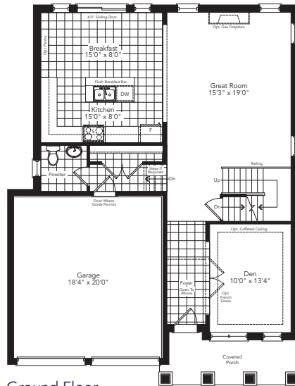
Ground Floor Elevation A
