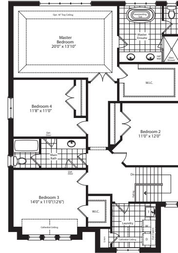
Optional Second Floor Plan Elevation A
