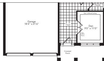
Partial Ground Floor Elevation B
