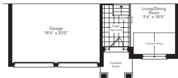
Partial Ground Floor Elevation B
