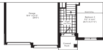
Partial Optional Second Floor 3 Bedroom Plan Elevation C
