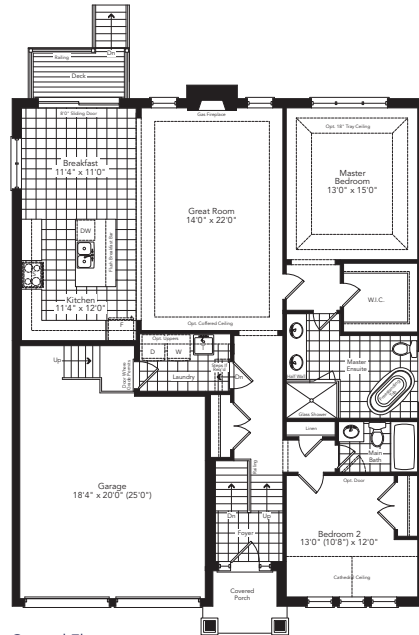
Ground Floor Elevation A
