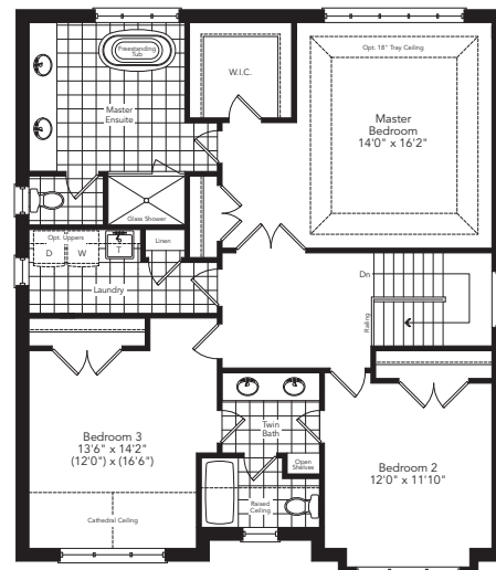
Second Floor Elevation A
