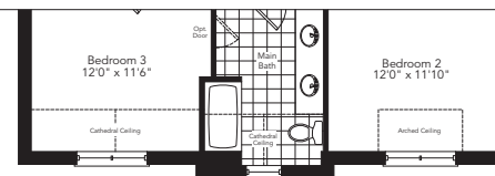
Partial Optional Second Floor 4 Bedroom Plan Elevation B
