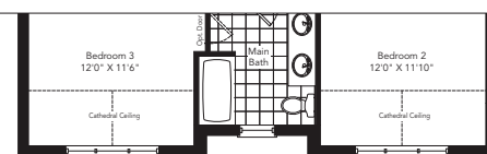
Partial Optional Second Floor 4 Bedroom Plan Elevation C
