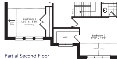
Partial Second Floor Elevation B
